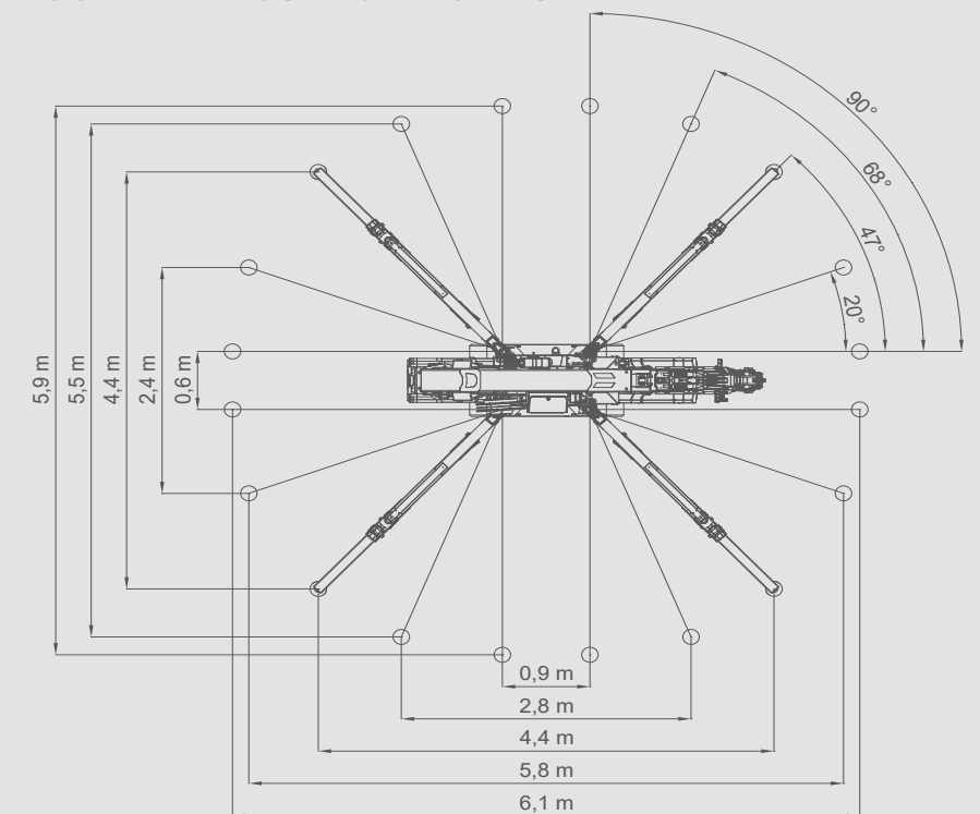
OUTRIGGER 2 ND POSITION FULL STABILITY
