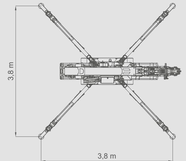
OUTRIGGER 2 ND POSITION FULL STABILITY
